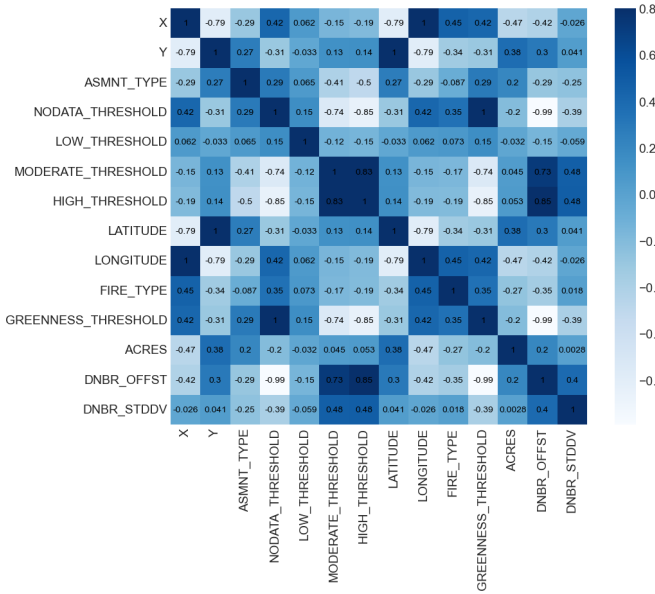
Fig. 2. Correlation Matrix
