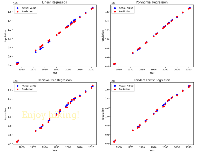
Fig. 2. Scatter plot of the Machine Learning Models
